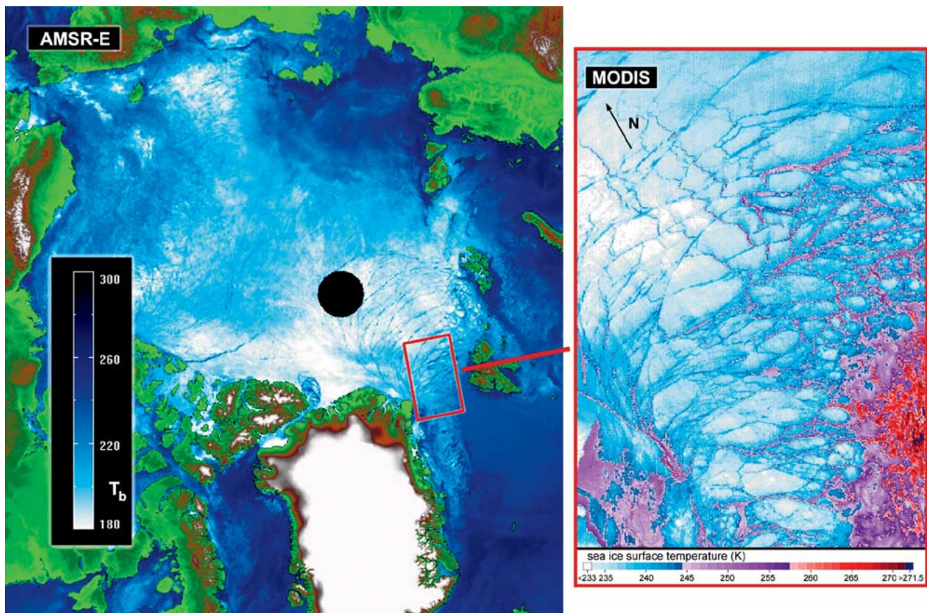
(Left) Advanced Microwave Scanning Radiometer-EOS 89-GHz vertically polarized image from the Aqua satellite, acquired on March 12, 2003, at a spatial resolution of \sim 5 km. (Right) Moderate-Resolution Imaging Spectroradiometer (MODIS) ice-surface temperature (IST) image, also acquired on March 12, 2003, but from the Terra satellite, showing part of the northern Greenland Sea. IST is provided as a MODIS standard product.
